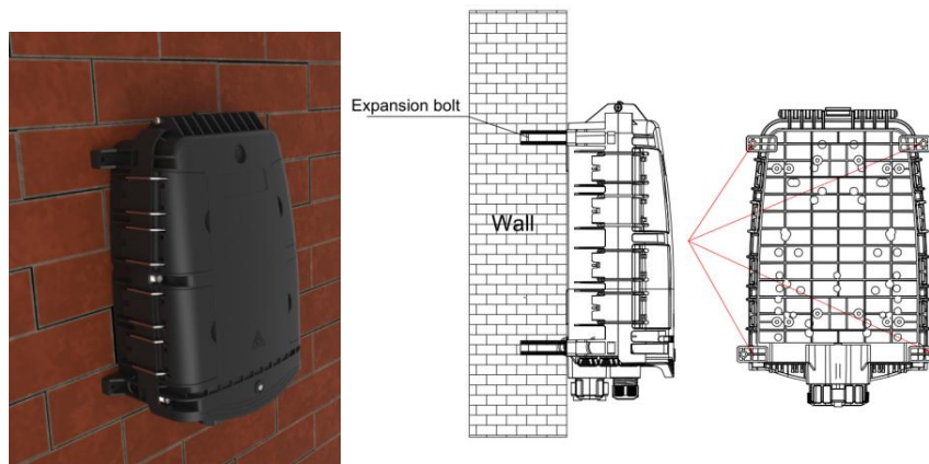
Wall mounted installation
