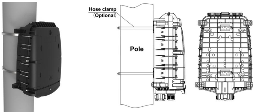
Pole mounted installation
